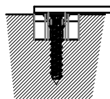
KARMFÆSTE 038290 MONTERET I 9X16 MM NOT. FIXING BRACKET 038290 FITTED IN 9X16 MM GROOVE
