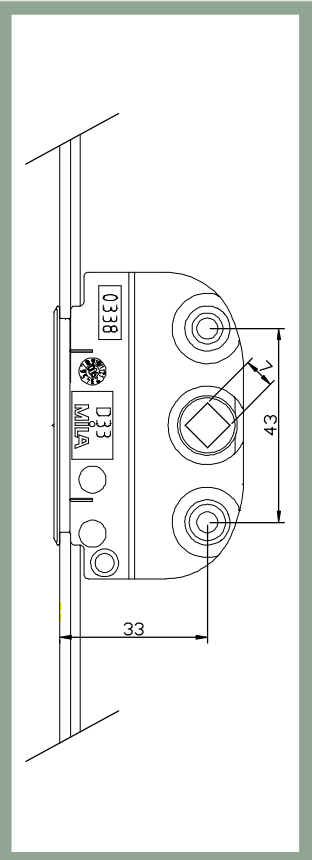
BACKSET 33 Z = 12 / 15 mm
