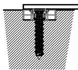
KARMFÆSTE 038291 MONTERET I 5X16 MM NOT. FIXING BRACKET 038291 FITTED IN 5X16 MM GROOVE
