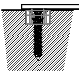
KARMFÆSTE 038292 MONTERET I 7X12 MM NOT. FIXING BRACKET 038292 FITTED IN 7X12 MM GROOVE
