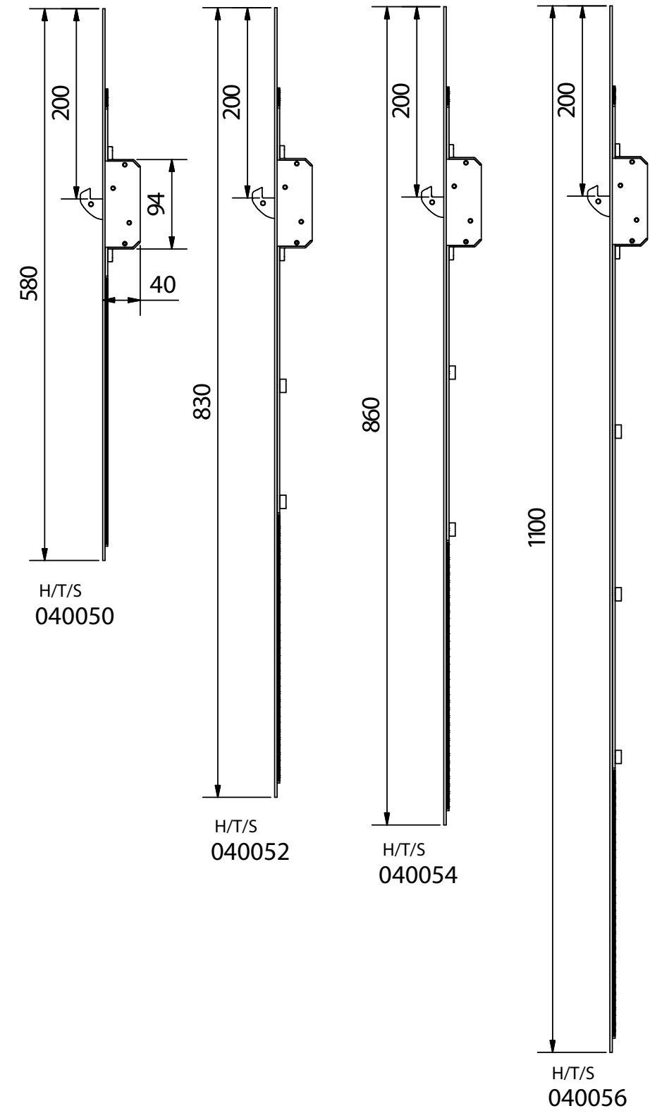
Top Extensions for Front Door, Patio and Stable Door Locks
