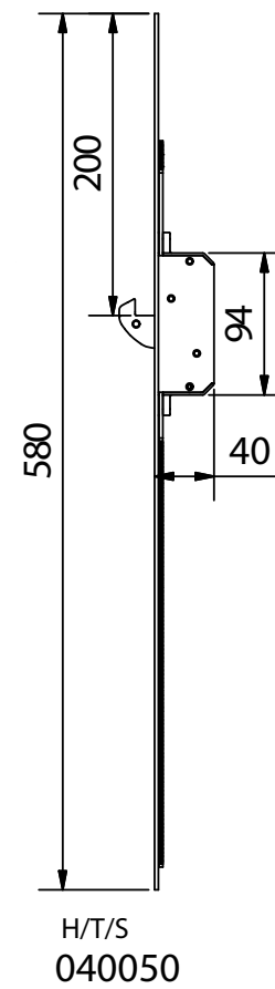
Top Extensions for Front Door, Patio and Stable Door Locks
