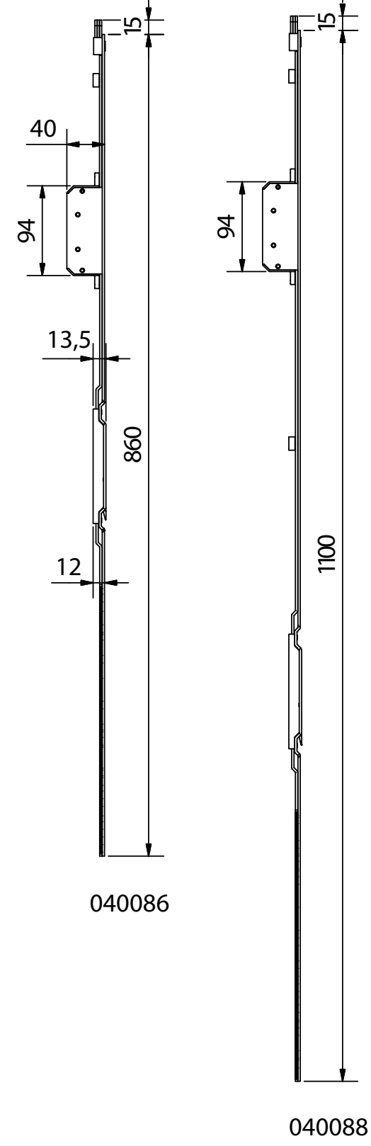
Top Extensions for Slave Doors
